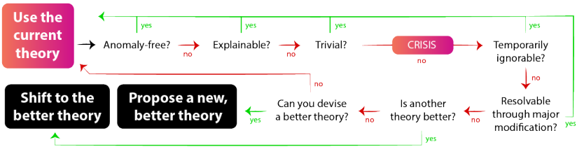
Fig. 2. An application of Kuhn's historical crisis cycles to our own theory adoption, creation, and rejection
